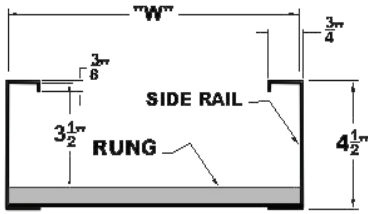
TRAY CROSS SECTION
