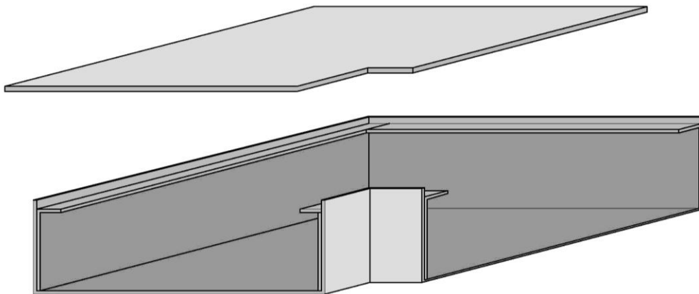
Figure 10: 6 inch Trench Duct Flat 90°
