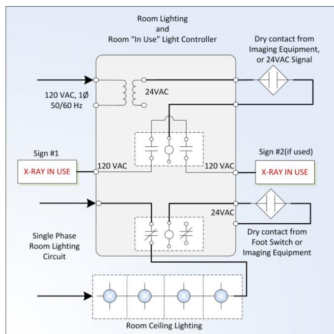
Figure 1 Nova Warning & Room Light Controller Application Diagram
