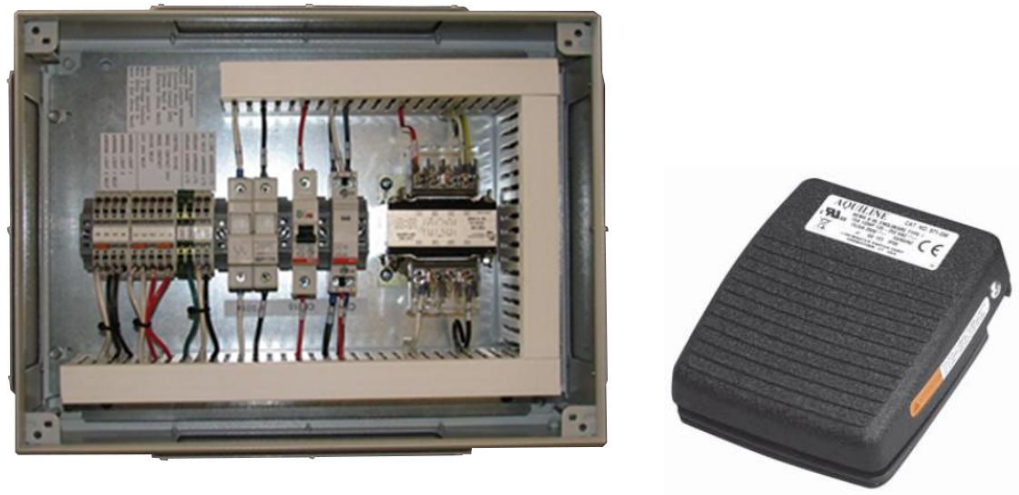
Figure 2 Nova Warning & Room Light Controller- Inside
